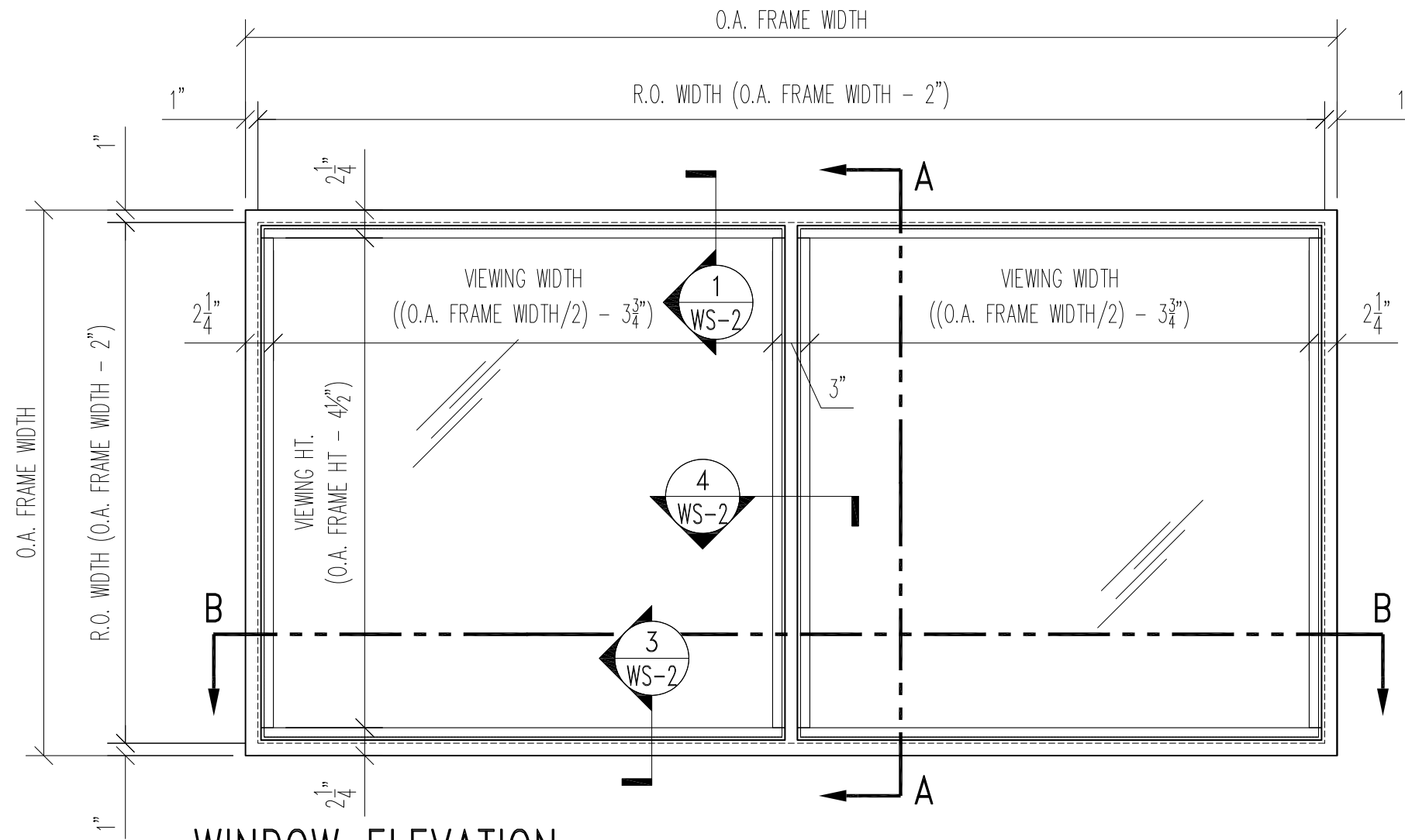
WINDOW ELEVATION
