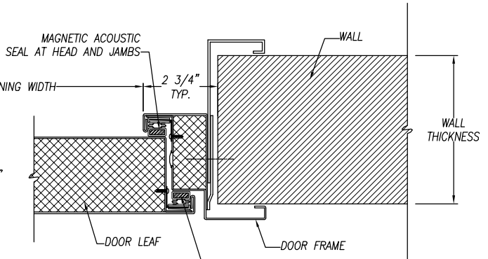
MAGNETIC ACOUSTIC SEAL AT HEAD AND JAMBS
