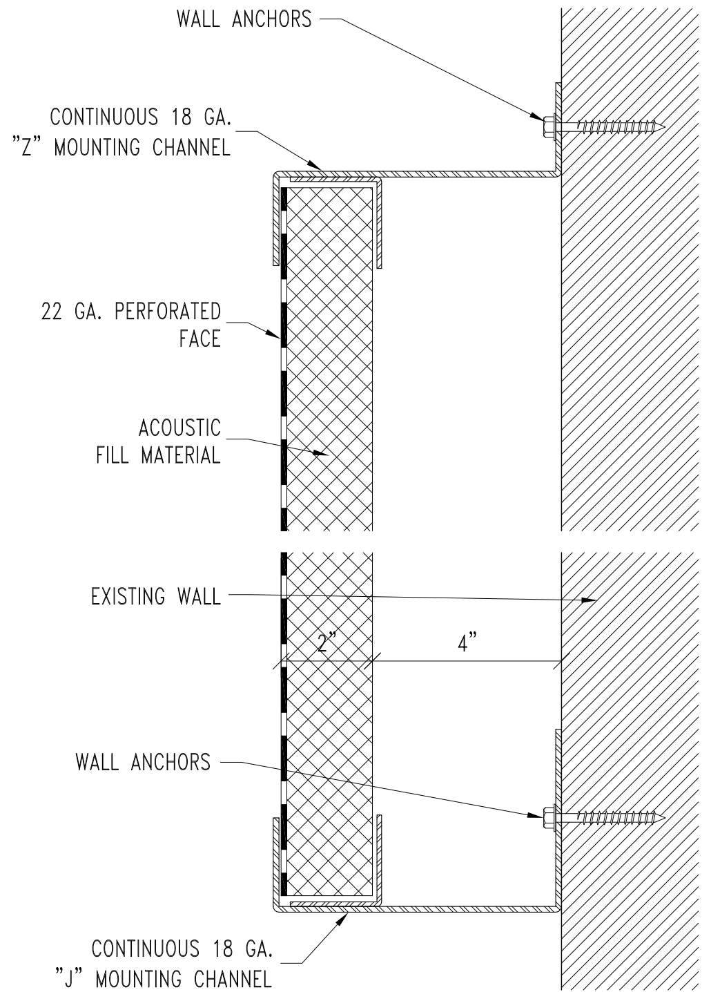
NB-II PANEL W/ 4" OFFSET
