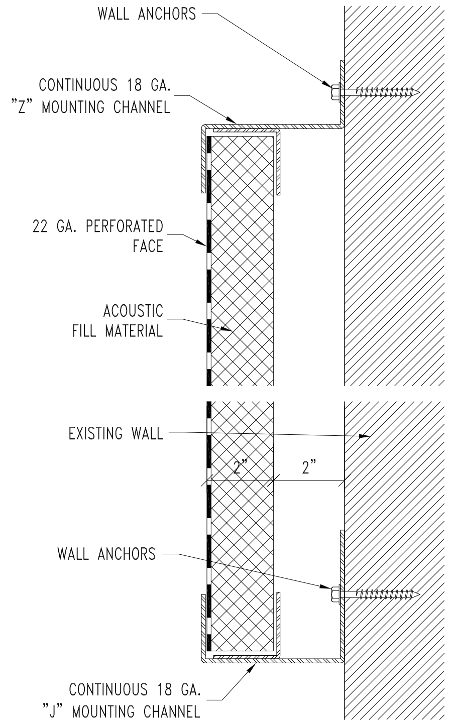
NB-II PANEL W/ 2" OFFSET
